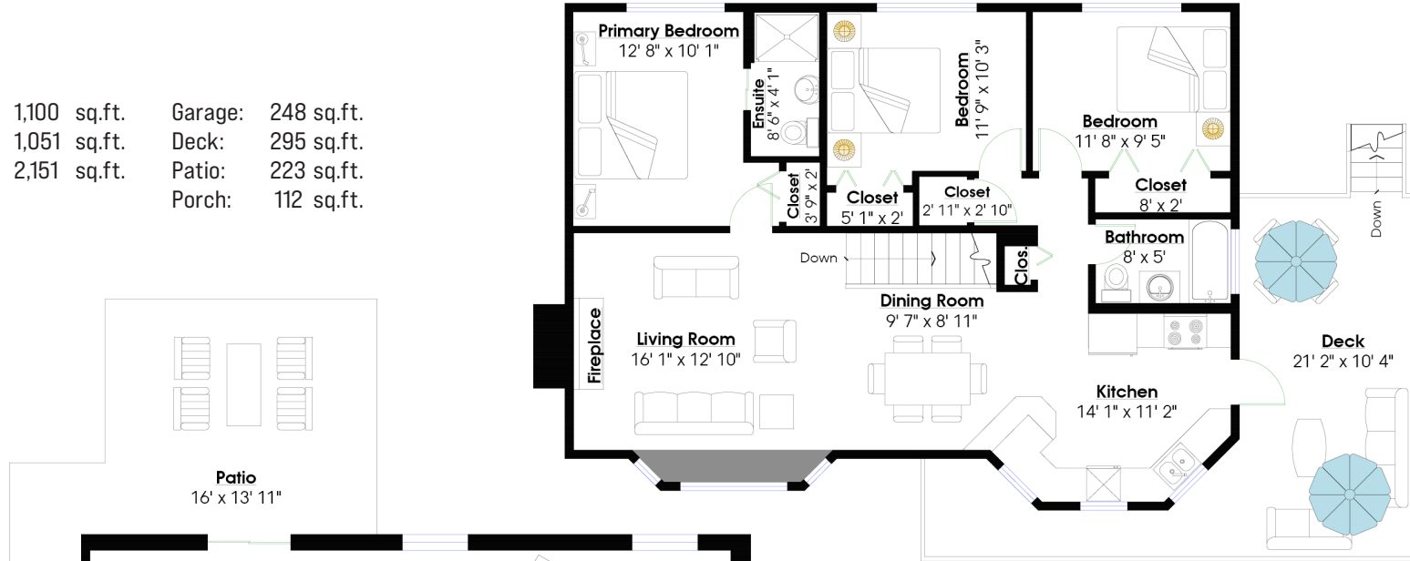
MAIN LEVEL Floor Area: 1,100 Sq. Ft. Ceiling Height: 8'
