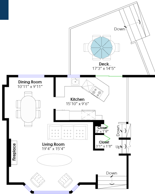
Floor Area: 691 Sq. Ft. Ceiling Height: 10'
