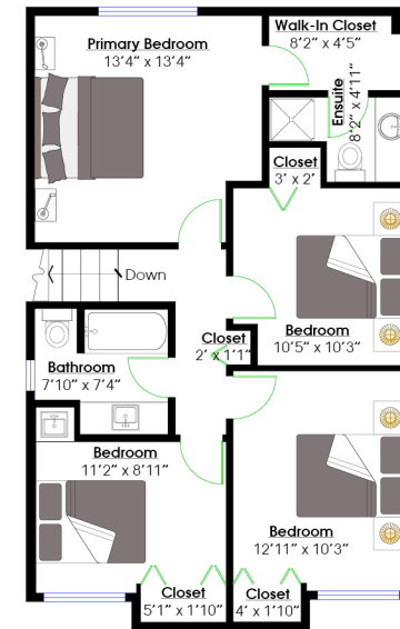
Floor Area: 816 Sq. Ft. Ceiling Height: 8'
